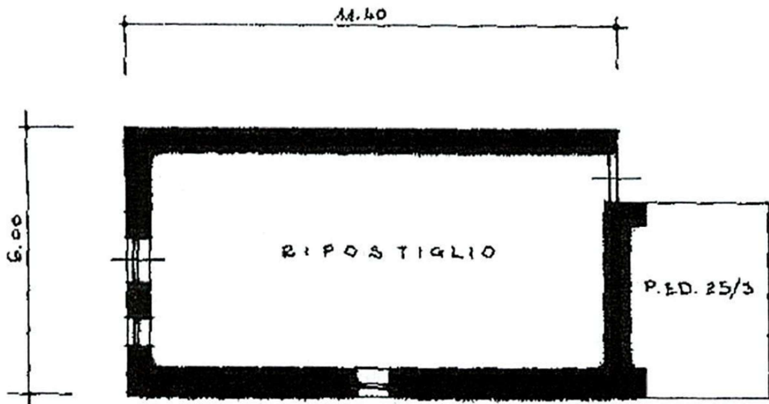
PIANO TERRA H: 2.10 ml.
