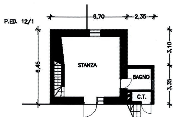
PIANO TERRA H = m 2,20
